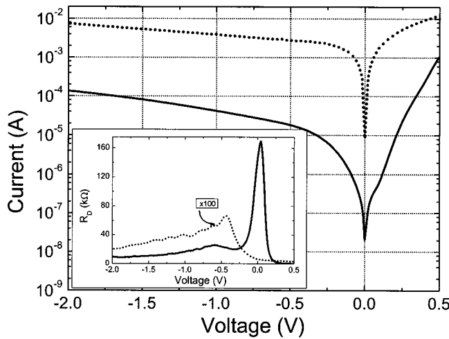
FIG. 1. Electrical characteristics of a PIN 30 μm diam InSb photodetector measured at room temperature (dotted line) and 77 K (solid line). The inset shows the calculated differential resistance.
