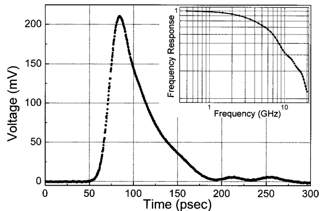
FIG. 4. Temporal response of a 30 μm PIN InSb photodetector measured at 2 V reverse bias. The inset shows the calculated FFT of this measurement where the 3 dB bandwidth is 7.5 GHz.
