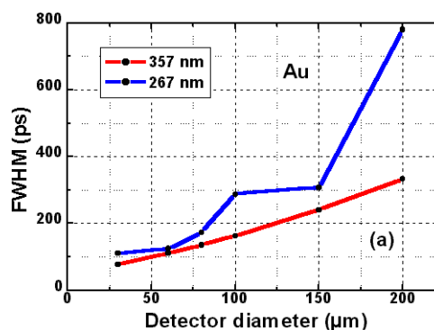
Figure 10a. Measured pulse-width variation with device area under 357 nm and 267 nm illumination. (a) Au-Schottky RCE-PD .
